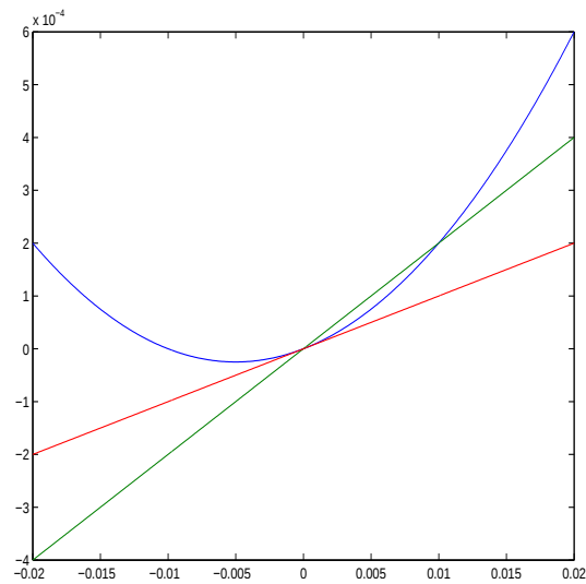
Figure 2: Plot of y = x^2 + 0.01x , y = 0.01x (tangent) and y = 0.02x (non-tangent)
