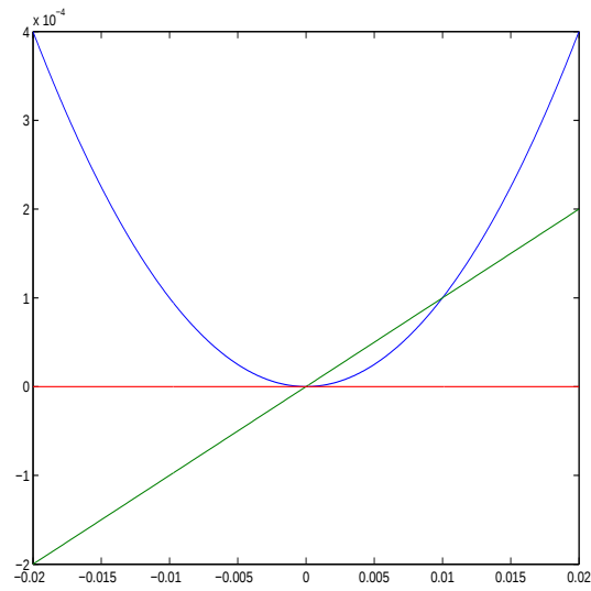
Figure 1: Plot of y = x^2 , y = 0 (tangent) and y = 0.01x (non-tangent)
