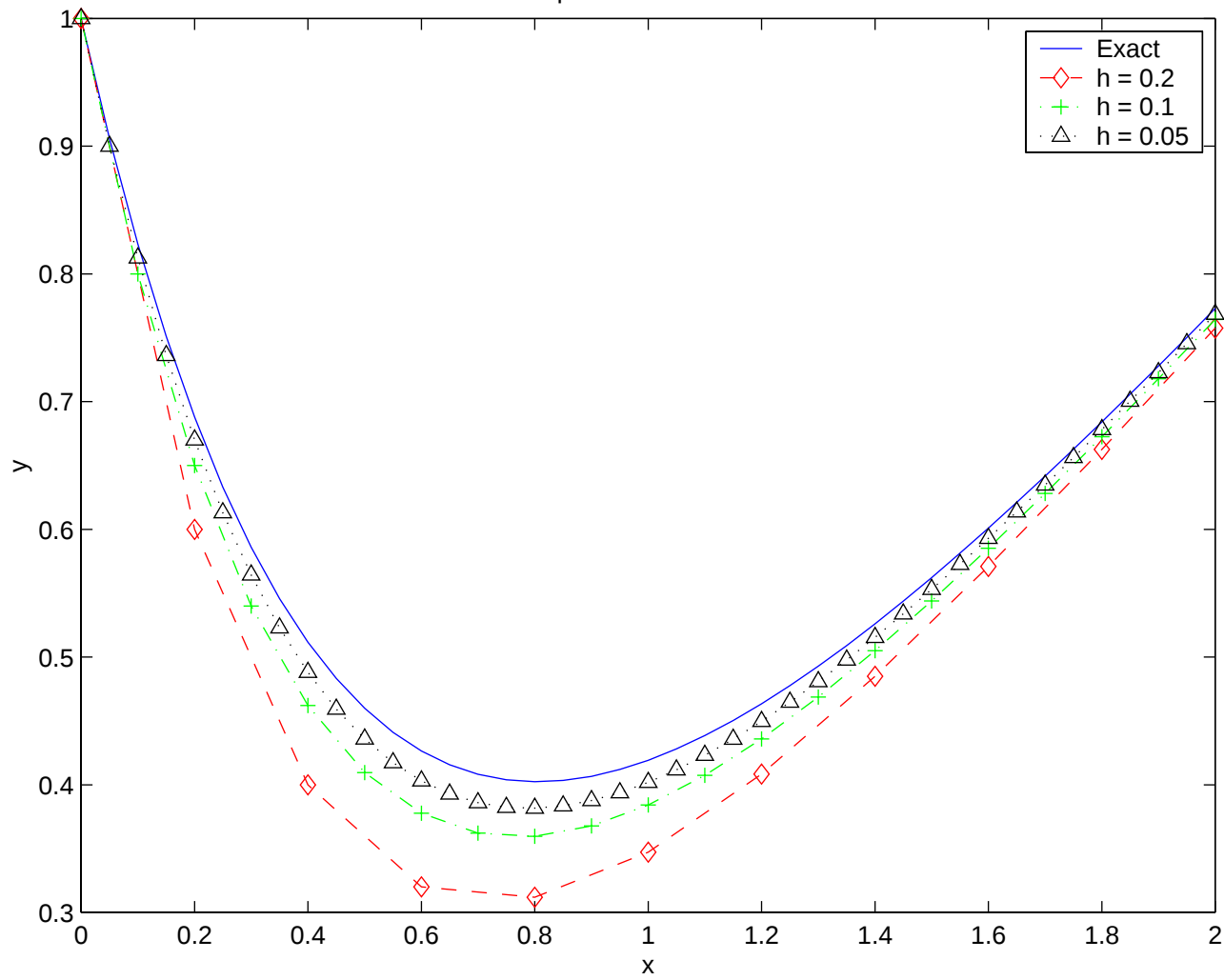
Example 1 for Euler method
