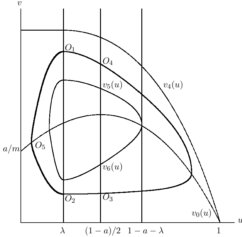
Figure 4: Illustration of the phase portrait (not up to scale) and the limit cycle in the proof. The isoclines are the thin solid curves: u = 0 , v = 0 , u = \lambda and the parabola v = v_0(u) ; the limit cycle is the thick solid curve O_1O_2O_3O_4 ; the boundary of the invariant region R_3 : v = v_4(u) is the outer boundary (together with u = 0 and v = 0 ; v = v_5(u) and v = v_6(u) are the upper and lower portions of inner boundary respectively; the line u = 1 - a - \lambda is the reflection of u = \lambda with respect to u = (1 - a)/2 .
