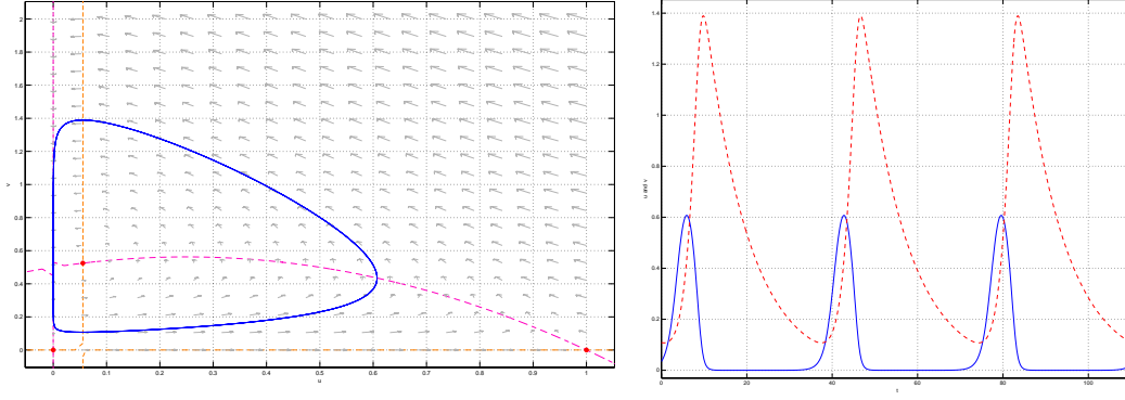
Figure 1: Plot of limit cycle. (left) phase portrait; (right) solution curves. Parameters: a = 0.5 , m = 1 , d = 0.1 , \lambda = 1/18 \approx 0.056 , period T \approx 37 .
