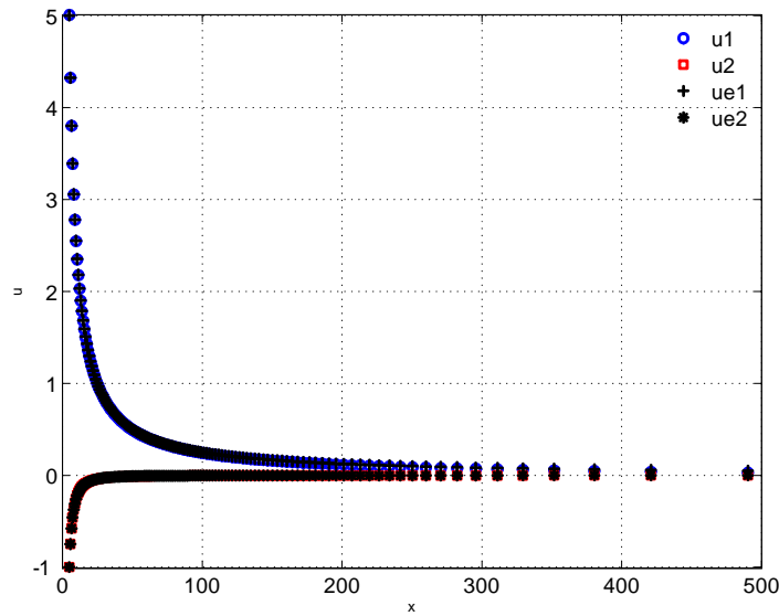
Figure 1: Sample exact and numerical solutions for the test problem (1). The symbols indicate: + the exact solution, • its first derivative, o the numerical solution, and □ its numerical first derivative.
