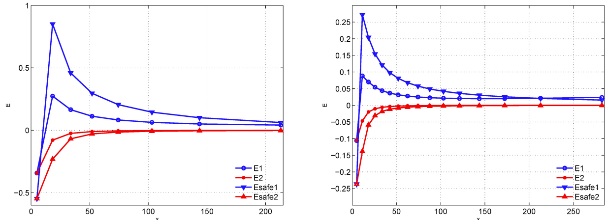
Figure 2: Safe error estimates provided by equation (15) and true error by equation (10) for the test problem (1). Here E_1 is the solution true error, E_2 true error for the solution first derivative, Esafe_1 the safe error estimate for the solution, and Esafe_2 the safe error estimate for the solution first derivative.
