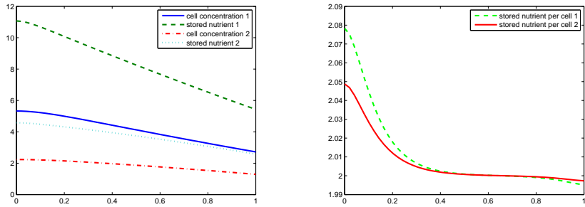
FIGURE 6. Profile of the coexistence steady state (left) and Q_1(x) , Q_2(x) (right) with growth and uptake functions as in (41) and (42). Here d = 0.01 . The horizontal axis is x ( 0 \leq x \leq 1 ), and the vertical axis is the value of functions.
